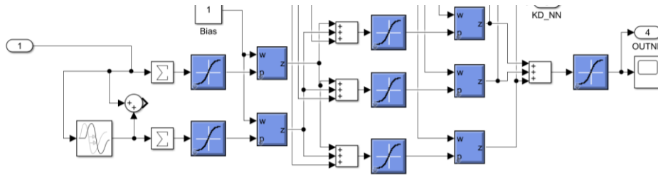
Figure 4. Artificial neural network architecture in RNNs
