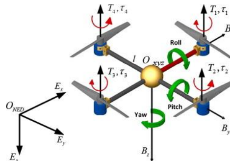
Figure 1. Quadcopter model [19]
